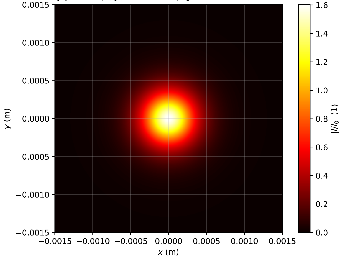
Intensity profile I(x, y, z = 2.707m)/I_0 , Pin=0.9Pcr, artificial time
